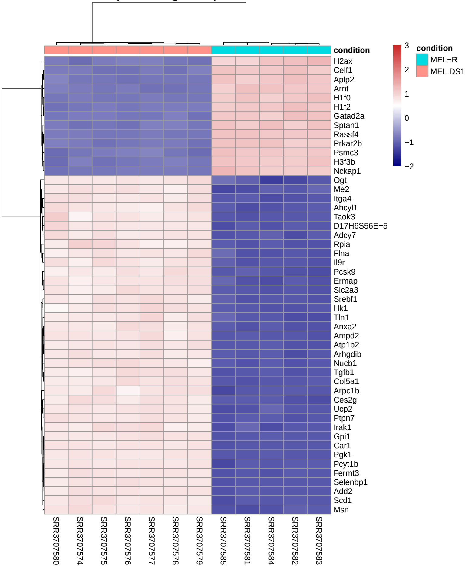
Replication Fig 1B: Top 50 Genes.
